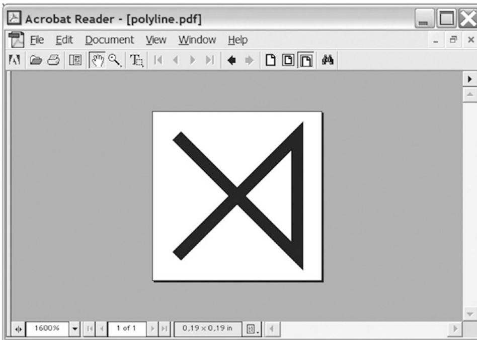
Figure 21-2. PolyLine([(0, 0), (10, 0), (10, 10), (0, 10)])
